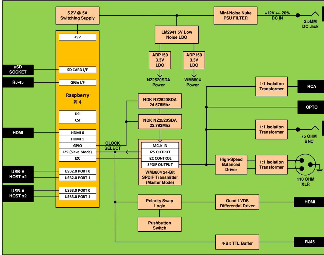
Figure 1 – MERCURY V3 Block Diagram
